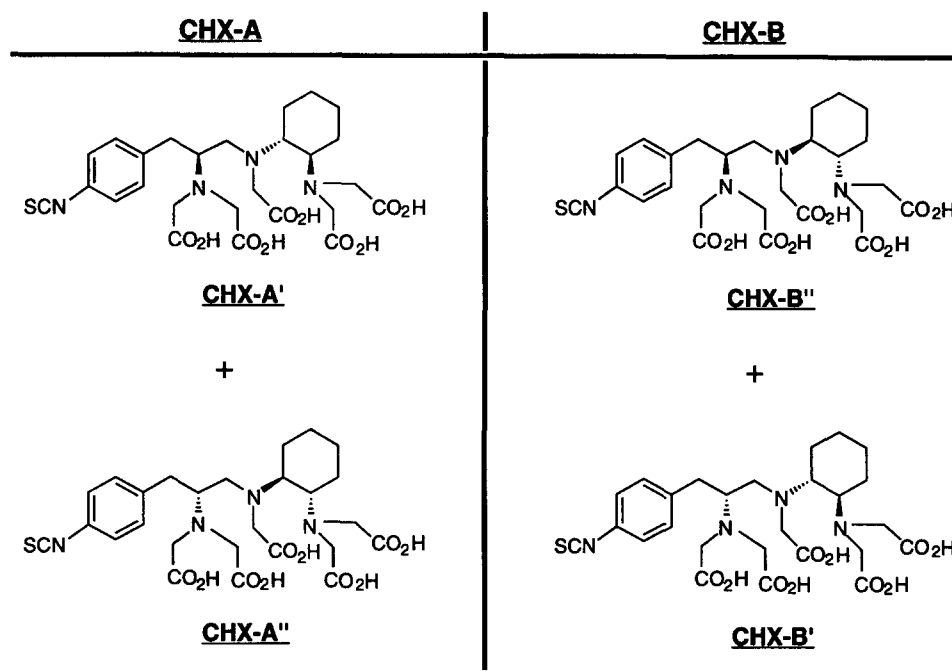
Figure 1. Structures of the CHX-A and CHX-B DTPA chelating agents and their individual component enantiomers.
