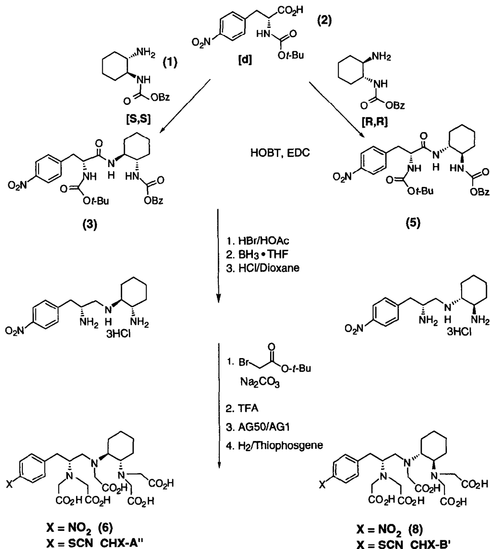
Figure 3. Stereospecific syntheses of the CHX-A'' and the CHX-B' DTPA chelating agents.
