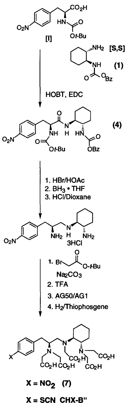
Figure 2. Stereospecific synthesis of CHX-B'' DTPA chelating agent.
