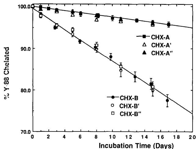
Figure 5. Serum stability of the ^{88}\text{Y} complexes of the four stereoisomers CHX-A', -A'', -B', B'' DTPA and their respective racemates over 17 days.
