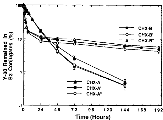
Figure 6. Transchelation of ^{88}\text{Y} from the ^{88}\text{Y} complexes of the four stereoisomers CHX-A', -A'', -B', B'' DTPA and their respective racemates conjugated to B3 versus excess EDTA.
