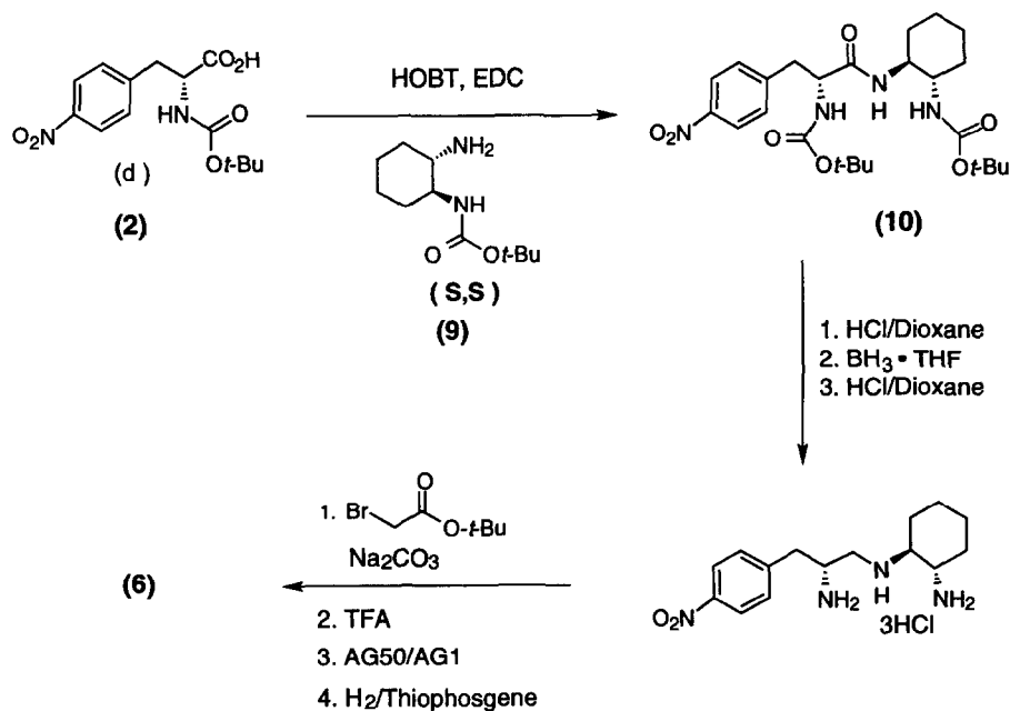
Figure 4. Modified stereospecific synthesis of the p -nitro precursor of CHX-A'' DTPA chelating agent.
